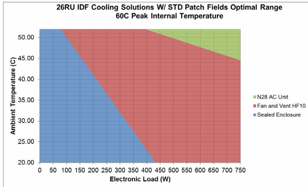
Figure 21: 26RU UDF enclosure guidelines for three recommended thermal solutions. The examples below demonstrate how to use this graph.
