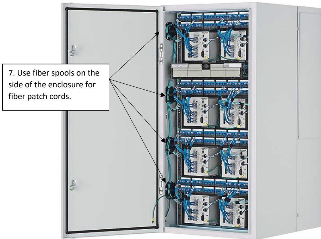
Figure 20 - A fully installed 26RU UDF
