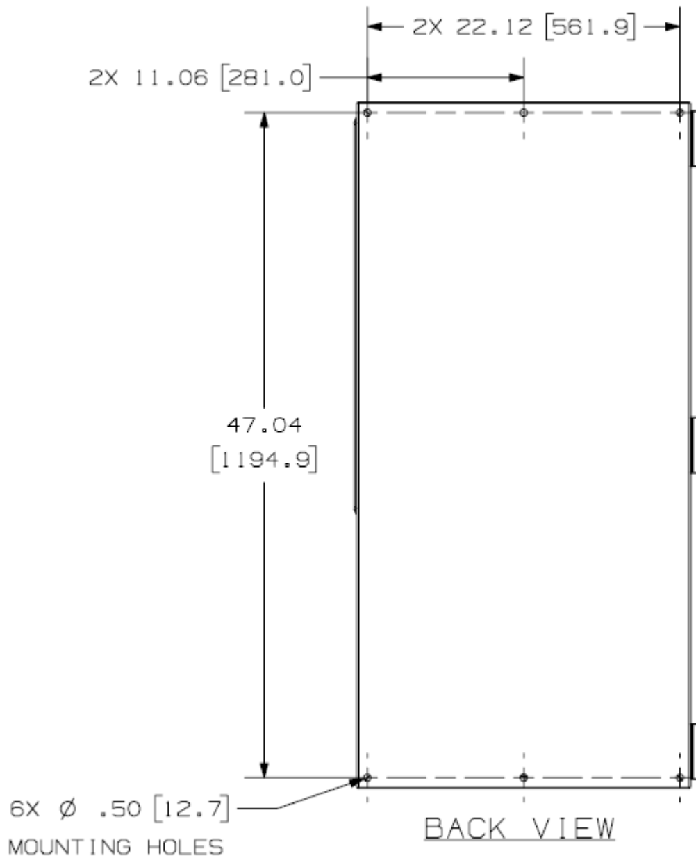
Figure 4: IDF Wall Section Mounting Holes
